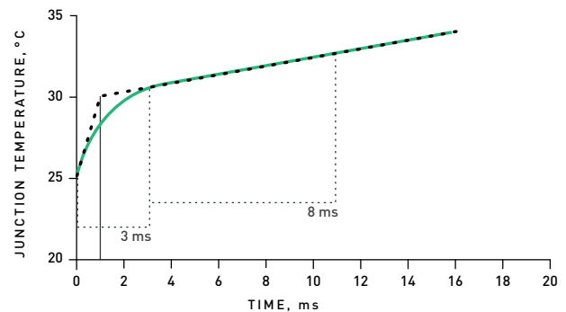
FIGURE 3: Crystal IS measures Klaran device power by waiting 3 ms after the start of the current pulse and then integrate the output for 8 ms.
