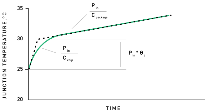
FIGURE 2: A simple model for the rise in junction temperature for a typical Crystal IS Klaran diode after power is applied to the device.
