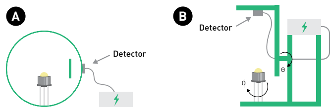
FIGURE 4: Typical measurement equipment for optical performance of LEDs—an integrating sphere (A) or a goniophotometer (B).
