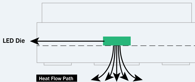
FIGURE A: Schematic of Crystal IS Klaran LED heat flow path
