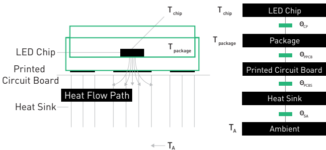
FIGURE 1: A simplified illustration indicating the Chip Temperature ( T_{chip} ), Package Temperature ( T_{package} ) and Ambient Temperature ( T_A ).
